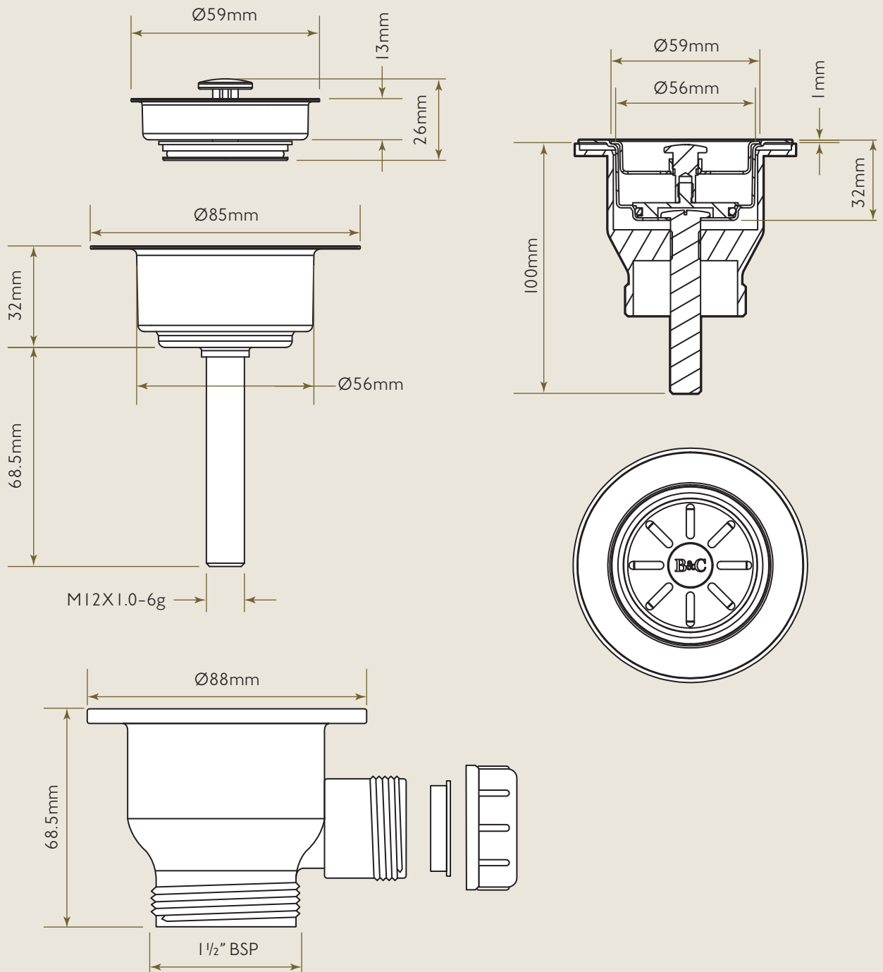
1.5" SOLID BRASS CONTEMPORARY WASTE
